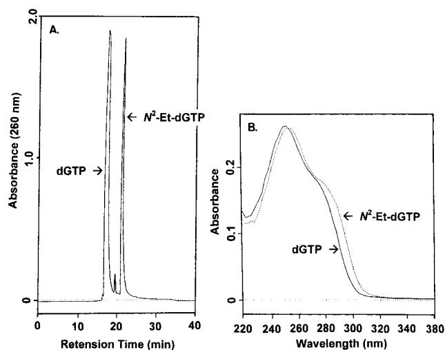
FIGURE 2: HPLC separation of N^2 -Et-dGTP. (A) dGTP was reacted with acetaldehyde in sodium acetate buffer, pH 4.5, and reduced by NaBaH 4 as described in the Material and Methods. N^2 -Et-dGTP was isolated from dGTP on a reversed-phase \mu Bondapak C 18 (0.39 \times 30 cm), using a linear gradient of 0.05 M triethylammonium acetate, pH 7.0, containing 0 \rightarrow 50% acetonitrile over 40 min and a flow rate of 1.0 mL/min. (B) UV spectra of N^2 -Et-dGTP and dGTP.
