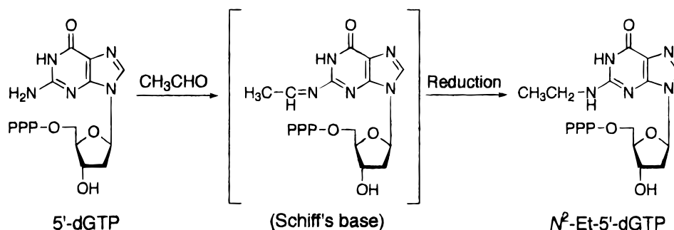
FIGURE 1: Formation of N 2 -Et-dGTP through Schiff's base.
