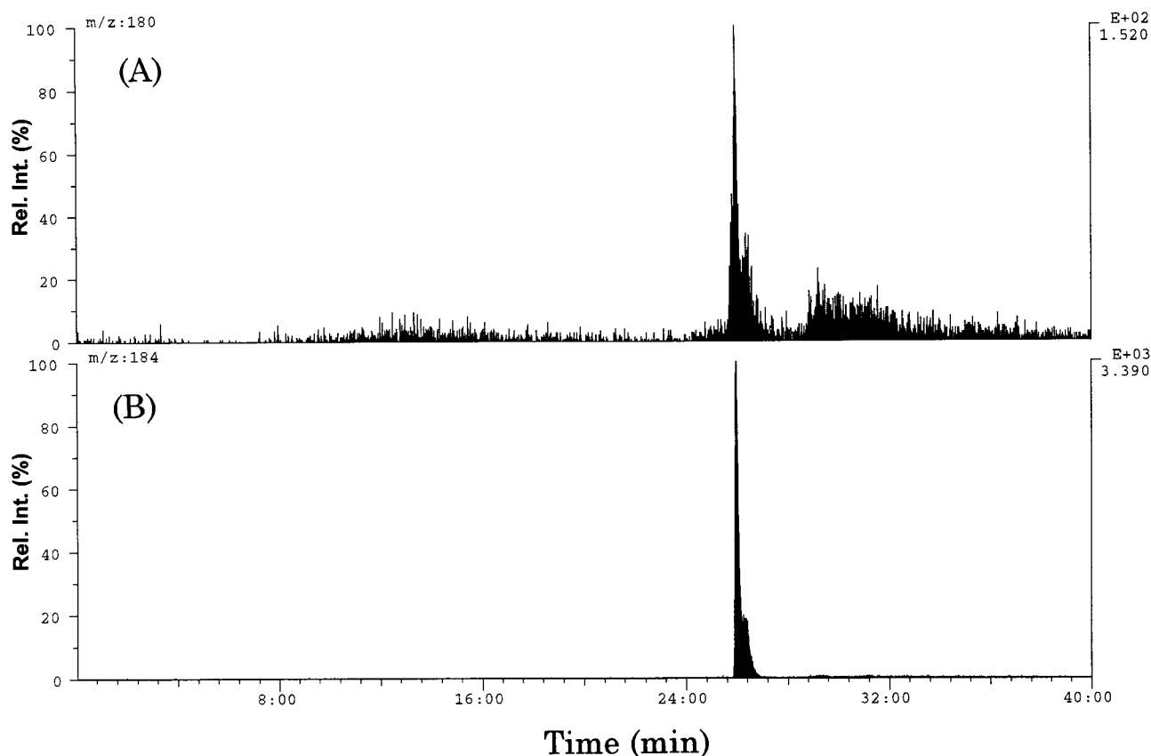
FIGURE 5: Detection of N^2 -Et-dG in human urine. A human urine sample containing N^2 -Et-dG- d_4 as an internal standard was analyzed by ESI/LC/MS/MS. The analytical condition was as described in Materials and Methods. Both N^2 -Et-dG (target) and N^2 -Et-dG- d_4 (internal standard) were analyzed by dual selected reaction monitoring (SRM) of (A) m/z 296 \rightarrow 180 for target N^2 -Et-dG and (B) m/z 300 \rightarrow 184 for internal standard N^2 -Et-dG- d_4 .
